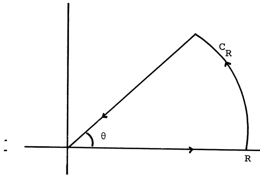
Figure 2. Contour of integration for (2.9).
