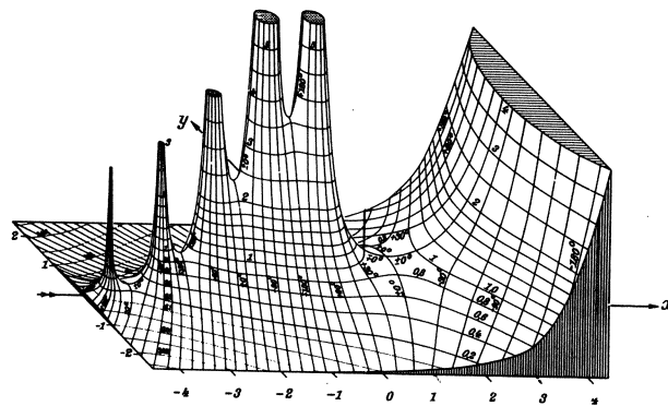
Figure 2. |\Gamma(z)| for complex z
