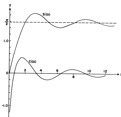
Figure 2. Graphs of \text{Si}(x) and \text{Ci}(x)
