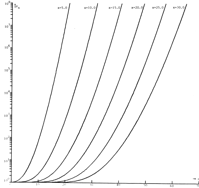
Figure 1. \rho_n of (3.1.23)
