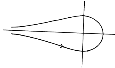
Figure 4 Contour for (1.6)
