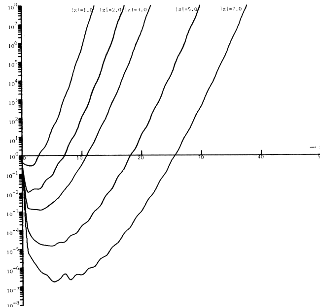
Figure 4. Graphs of (3.1.30)
